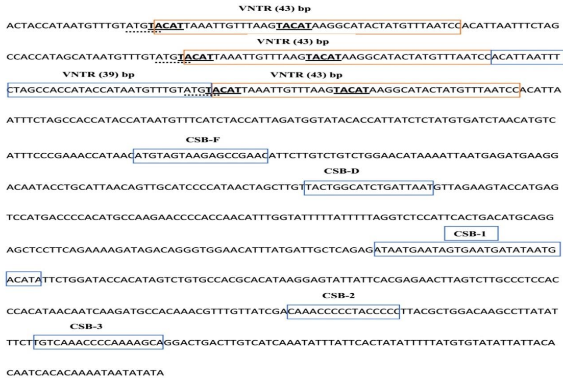
Fig. 3. The structure of control region in A. persicus . The dashed and simple lines depict the reversed complement cTAS (ATGTA) and TAS (TACAT) motifs, respectively. Central conserved sequence block domains (CSB-D and CSB-F), three conserved sequence block domains (CSB-1, CSB-2, and CSB-3), and the variable number of tandem repeats are in the boxes.
