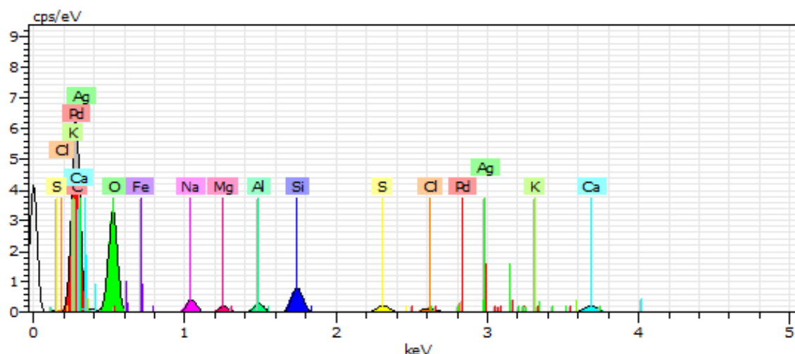
Fig. 6. EDS spectra of S. portulacastrum leaf represented interaction between Ag and Pb (100 mg L -1 ).
