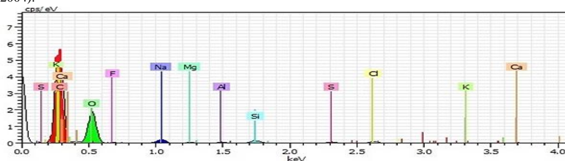
Fig. 3. EDS spectra of S. portulacastrum leaf control (100 mg L -1 ).
