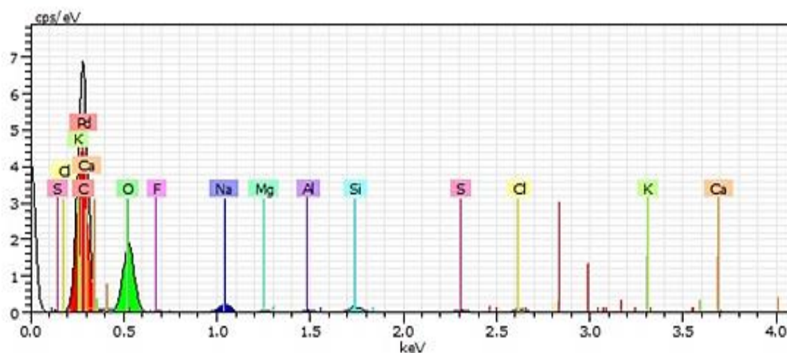
Fig. 4. EDS spectra of S. portulacastrum leaf treated with Pb (100 mg L -1 ).
