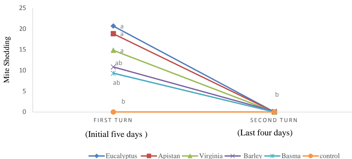
Fig. 2. The interaction effect of time and the use of anti-mite substances (Eucalyptus extract, Virginia, Barley and Basma tobacco smoke and Apistan strip) in two turns (first: initial five days and second: last four days) with 25 days interval on Varroa mite shedding (LSMeans ± SE)
