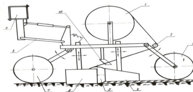
Fig. 1. Structural and technological scheme of the film-laying unit section; 1 – film roll; 2 – guide; 3 – pressing device; 4 – covering discs; 5 – press roller; 6 – soil deflector; 7 – support wheel; 8 – section suspension; 9 – frame; 10 – blades.
