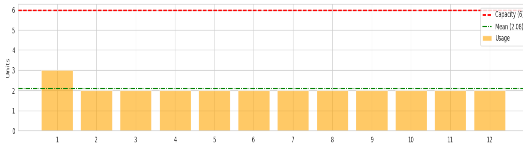
Figure 2: Utilization profile for Resource R_1 (Engineers); the minimal deviation from the mean (2.08) confirms the quadratic objective's ability to smooth workforce demand under a capacity of 6.
