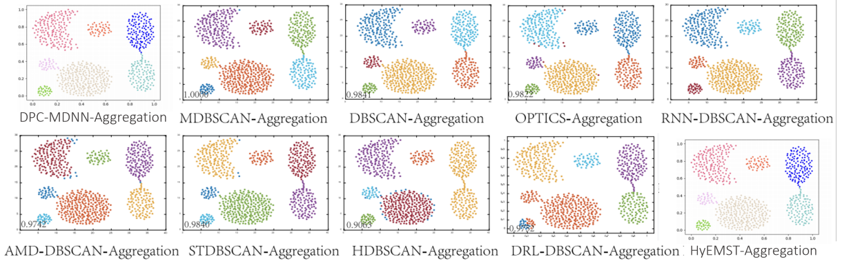
Figure 3: Clustering results on Aggregation dataset (arbitrary shapes and sizes). HyEMST output showing perfect recovery ( \text{NMI}=\text{ARI}=1.0 ). Ellipsoidal volumetric density estimation adapts to anisotropic micro-clusters, enabling robust MST-based merging on irregular geometries.
