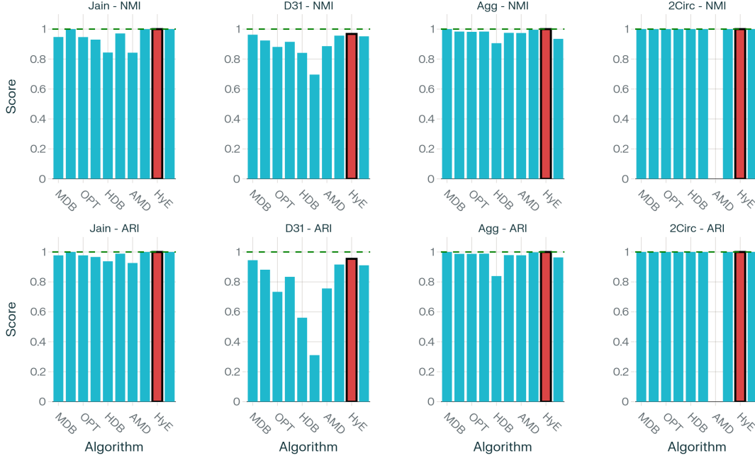
Figure 5: Comparative performance visualization across synthetic datasets. Bar plots report NMI (top) and ARI (bottom) for representative baselines and HyEMST on Jain, D31, Aggregation, and 2Circles. HyEMST consistently attains perfect or near-perfect scores across diverse geometric and density regimes; dashed lines indicate the optimum score of 1.0.
