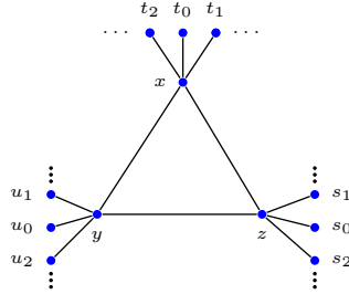
Figure 3: The planar Corona product graph K_3 \circ \overline{K}_{|\mathfrak{q}_t \setminus \mathfrak{q}_s \cup \mathfrak{q}_r|} for each 1 \leq r, s, t \leq 3 .
