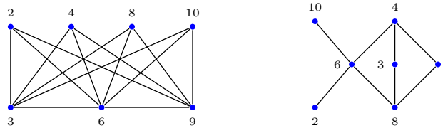
Figure 7: The non-planar graph EG(\mathbb{Z}_{12}) and the planar graph \Gamma(\mathbb{Z}_{12}) .
