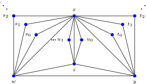
Figure 1: The planar graph EG(\mathcal{M}) = P_1 \vee (K_{1,|\mathfrak{q}_1 \setminus r(\text{Ann}_{\mathcal{R}}(\mathcal{M}))|} \cup K_{1,|\mathfrak{q}_2 \setminus r(\text{Ann}_{\mathcal{R}}(\mathcal{M}))|} \cup K_{1,|\mathfrak{q}_3 \setminus r(\text{Ann}_{\mathcal{R}}(\mathcal{M}))|}) .
