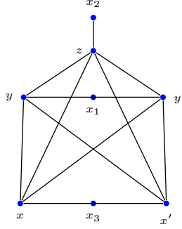
Figure 2: The non-planar graph EG(\mathcal{M}) with |\mathfrak{q}_1 \cap \mathfrak{q}_3| = |\mathfrak{q}_2 \cap \mathfrak{q}_3| = 2 .
