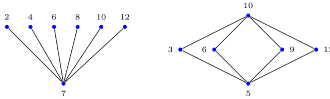
Figure 6: The planar zero-divisor and the essential graphs \mathbb{Z}_{14} and \mathbb{Z}_{15} .
