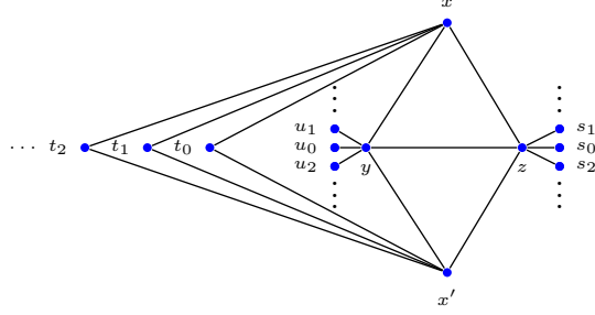
Figure 4: The planar graph EG(\mathcal{M}) = (K_3 \circ \overline{K}_{|q_t \setminus q_s \cup q_r|}) \cup (K_3 \circ \overline{K}_{|q_t \setminus q_s \cup q_r|}) .
