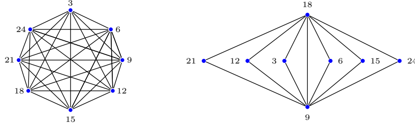
Figure 5: The non-planar graph EG(\mathbb{Z}_{27}) and planar graph \Gamma(\mathbb{Z}_{27})
