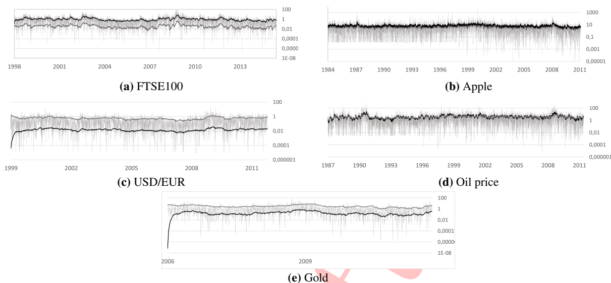
Figure 1: Realized volatility measured by squared returns (light gray) and estimated volatility from ASV (black) and ALGARCH (dark gray) for daily financial return series (y-axis on a logarithmic scale)
