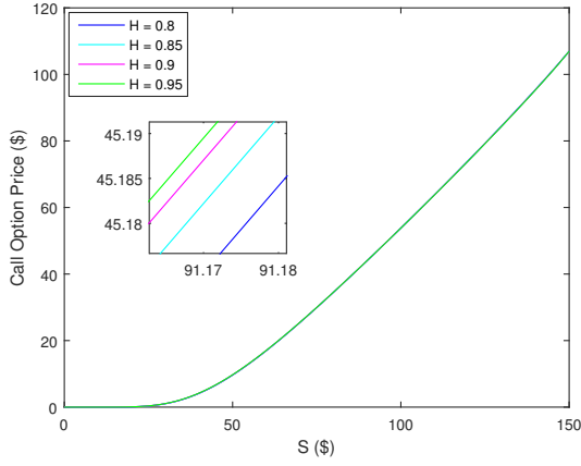
Figure 11: American option price based on different H when N = M = 100
