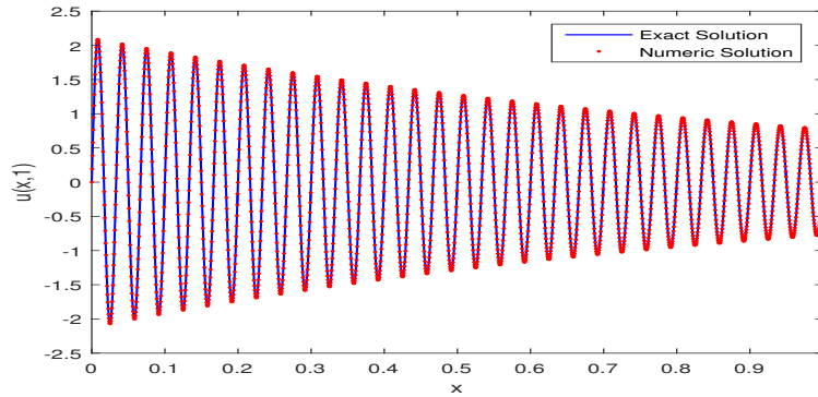
Figure 9: Comparison of the exact solution with the approximation solution obtained from the proposed method when \alpha = 0.75 , \lambda = 1 , \mu = 0 and N = 256 , M = 256 , t = 1 , k = 30 for Example 4
