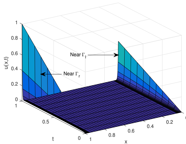
Figure 2: Rotated version of Figure 1
