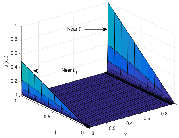
Figure 1: Solution profile u(x,t) of Example 1
