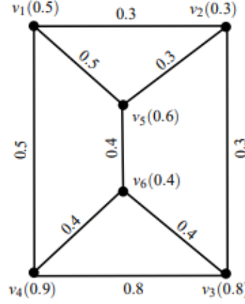
Figure 4: Fuzzy graph G demonstrating perturbation.
