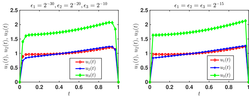
Figure 4: Solution plots of Example 2 for N = 64 .
