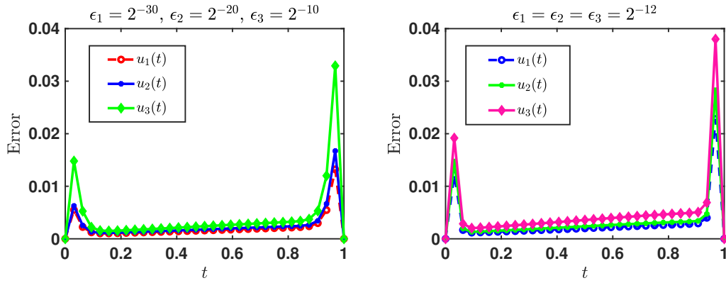
Figure 5: Error plots of Example 2 for N = 64 .
