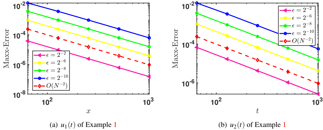
Figure 3: Log-log plot with corresponding values of \epsilon = \epsilon_1 = \epsilon_2 .
