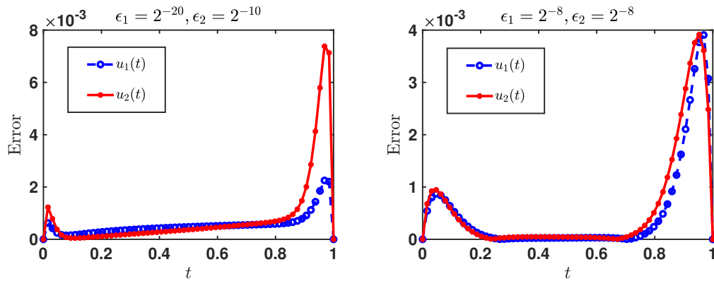
Figure 2: Error plots of Example 1 for N = 64 .
