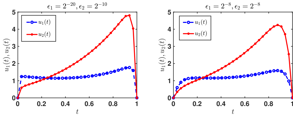
Figure 1: Solution plots of Example 1 for N = 64 .
