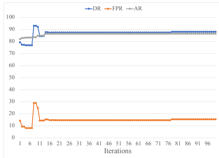
Figure 6: Convergence diagram of the proposed method for the NSL-KDD dataset.
