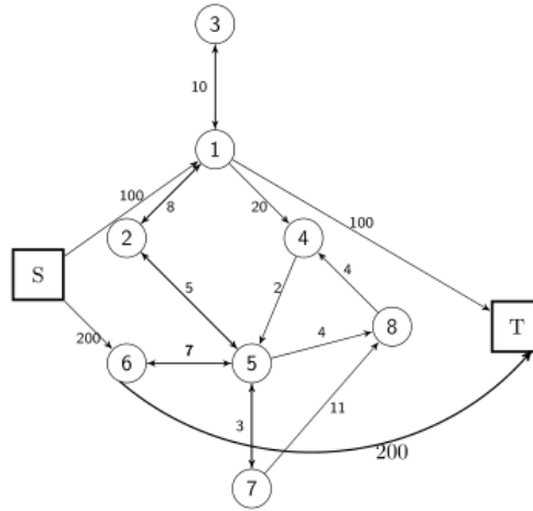
Figure 4: An example of a directed non-complete graph
