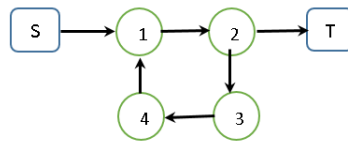
Figure 3: Arc (1,2) must be passed twice
