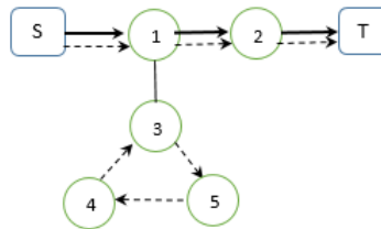
Figure 2: An example for disconnected subtour
