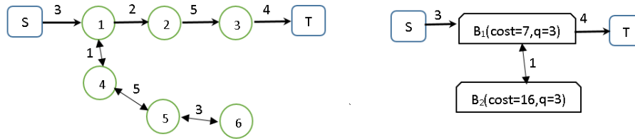
Figure 5: An example for the blocking procedure
