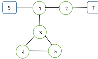
Figure 1: An example for non-complete graph
