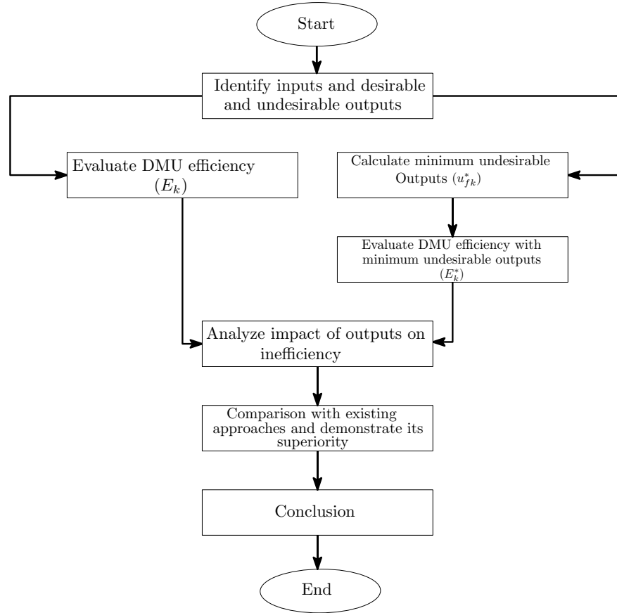
Figure 1: Research framework
