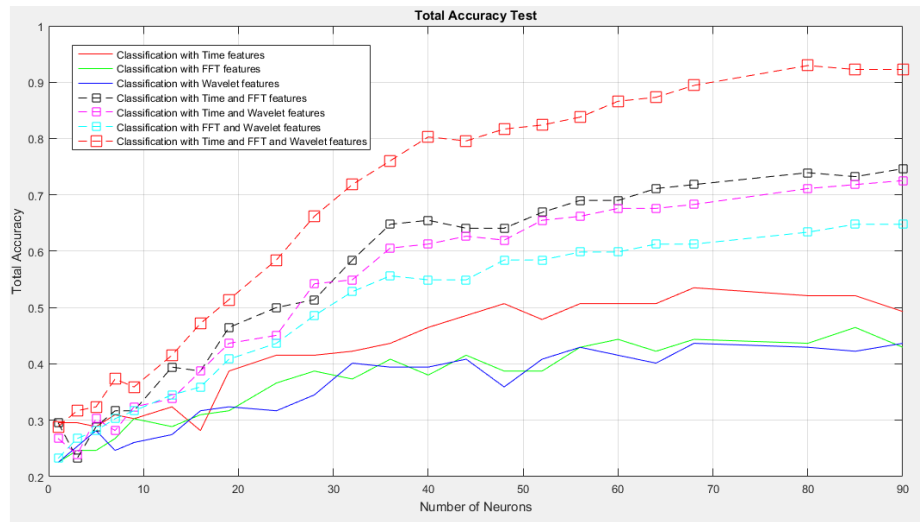
Figure 8 Accuracy classification results with various kind of features and neurons numbers.
