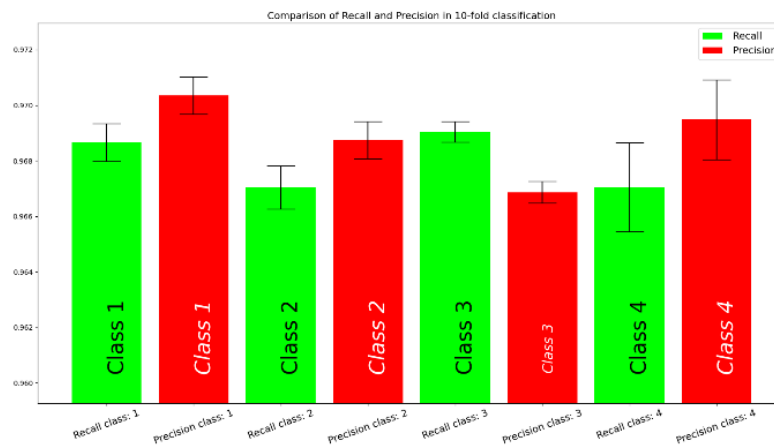
Figure 11 Mean and variance of 4 groups in the 10-fold method using deep learning classification.
