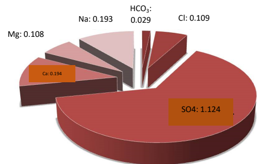
Fig. 3. Indicators of salts in the soil of experimental plot B-71-8.
