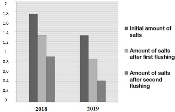
Fig. 4. Dynamics of plot flushing norms.
