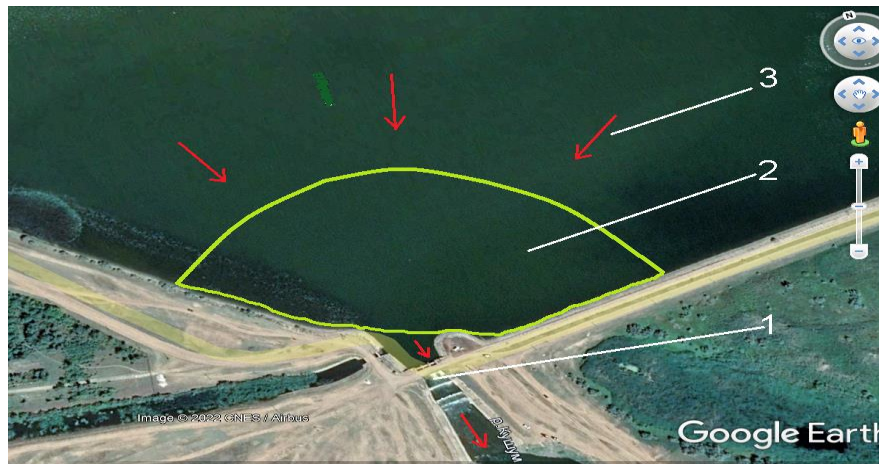
Fig. 2. Section of the water area in front of the spillway, at a distance of 150 m from the gate valve, dangerous for fish and juveniles (1 - dam spillway; 2 - section of the water area dangerous for fish and juveniles; 3 - direction of flow).
