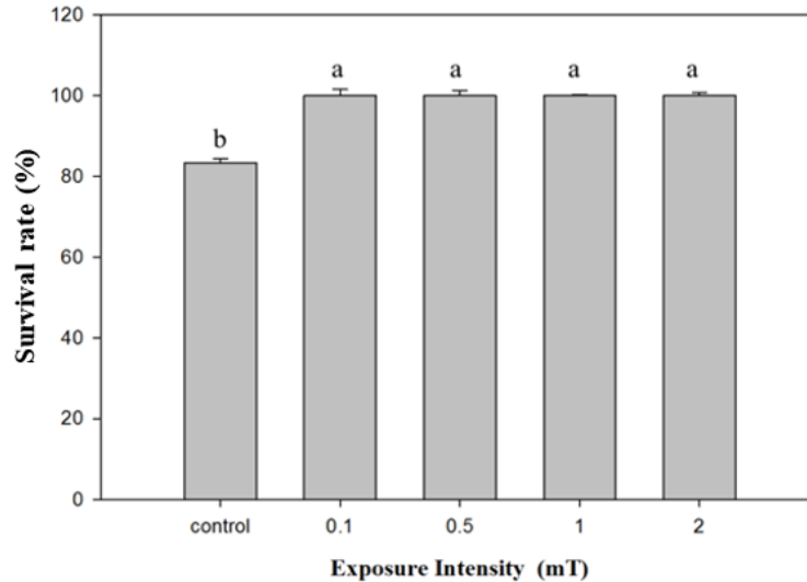
Fig. 2. Survival rate of common carp fingerling after 60 days acute exposure at different intensities of ELF-EMF. Different superscript letters indicate significant ( P < 0.05 ) differences of the means.
